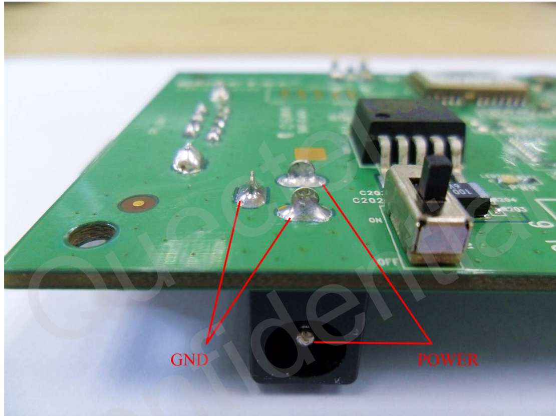
Figure 4: Power interface
