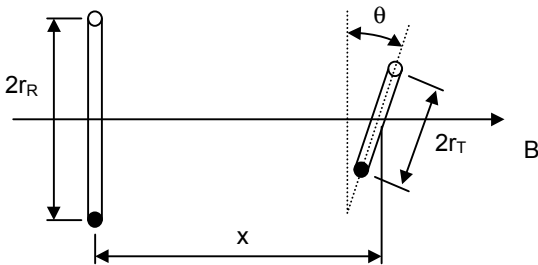
Figure 10: Parameters influencing the coupling factor k
