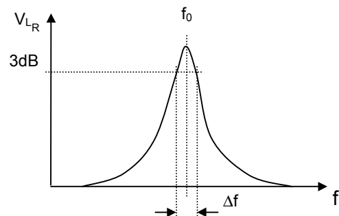
Figure 12: Series resonance curve
