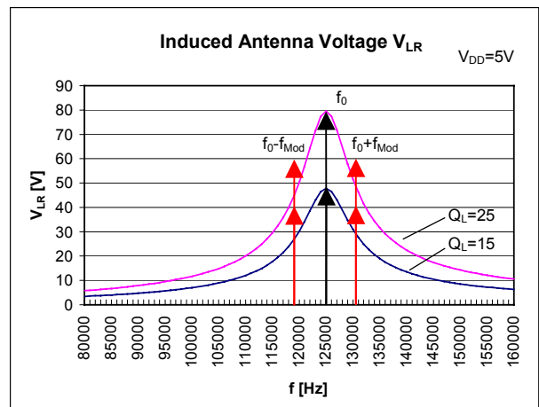
Figure 14: Induced antenna voltage
