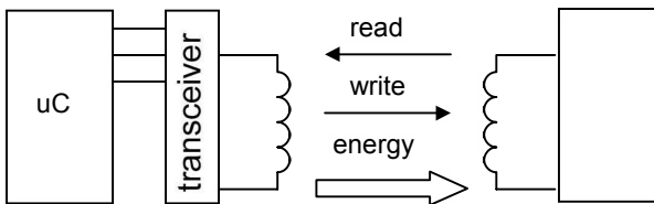
Figure 4: Basic RFID system setup
