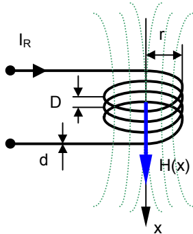
Figure 6: A short cylindric coil
