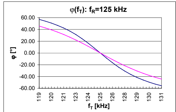
Figure 13: Phase shift \varphi between two resonant circuits
