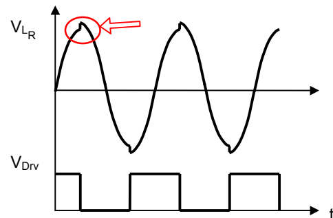
Figure 17: Tuning the resonance circuit
