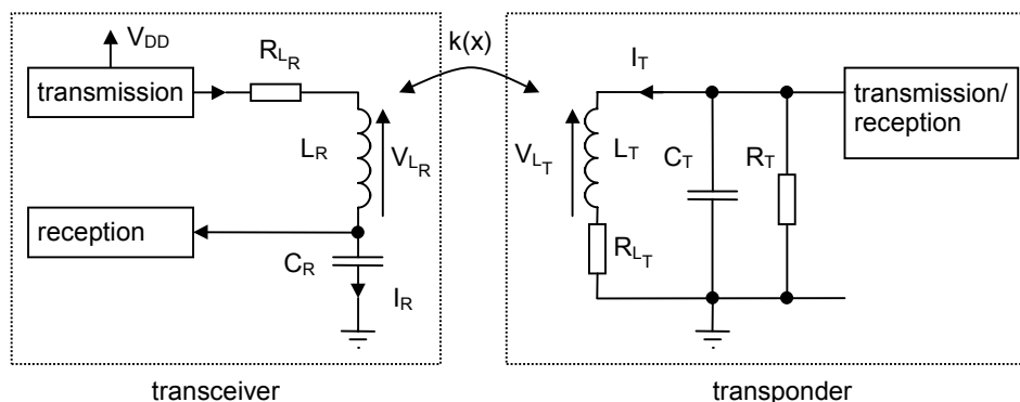
Figure 5: RFID system frontend [B4]
