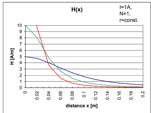
Figure 8: Normalised H(x) with three different reader antenna diameters
