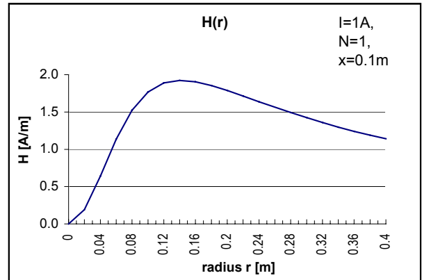
Figure 7: The magnetic field strength H(r)
