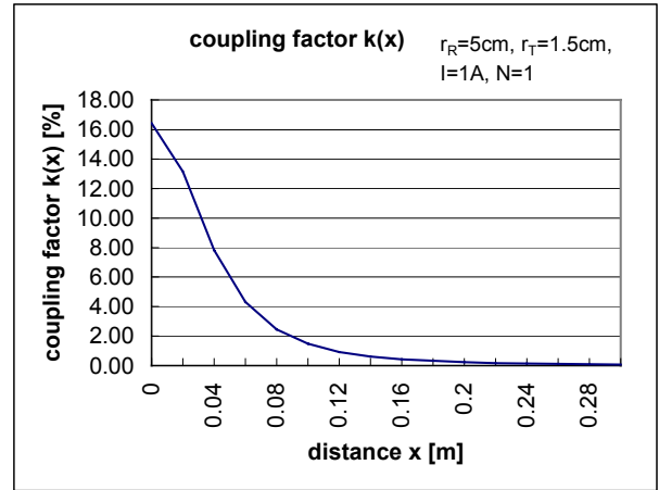
Figure 11: Magnetic coupling factor k for a fixed antenna setup
