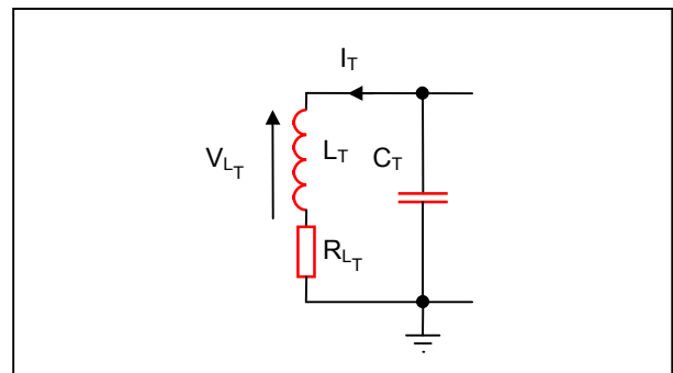
Figure 16: Parallel resonance circuit at the transponder side
