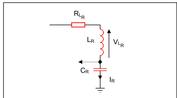
Figure 15: Series resonance circuit at the reader side
