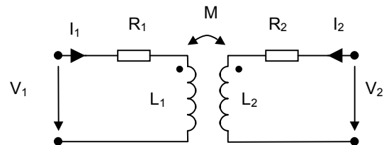
Figure 9: Transformer model
